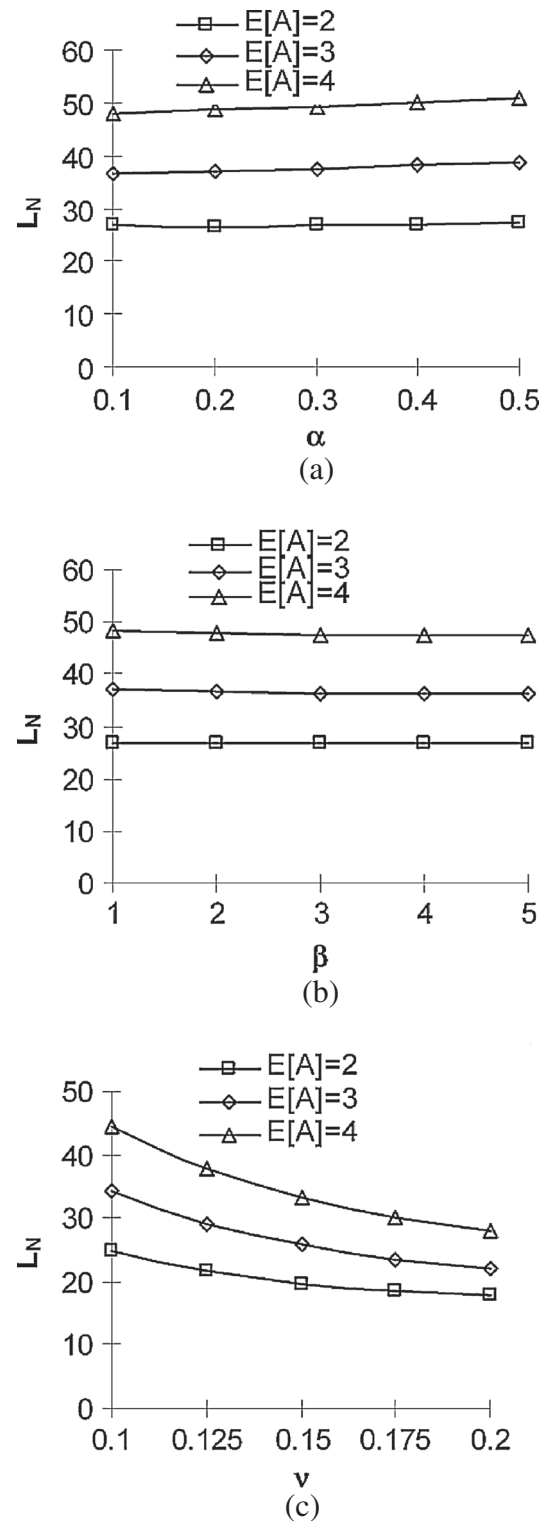
Figure 2 Average queue length vs. (a) \alpha , (b) \beta , and (c) v for different batch sizes.
