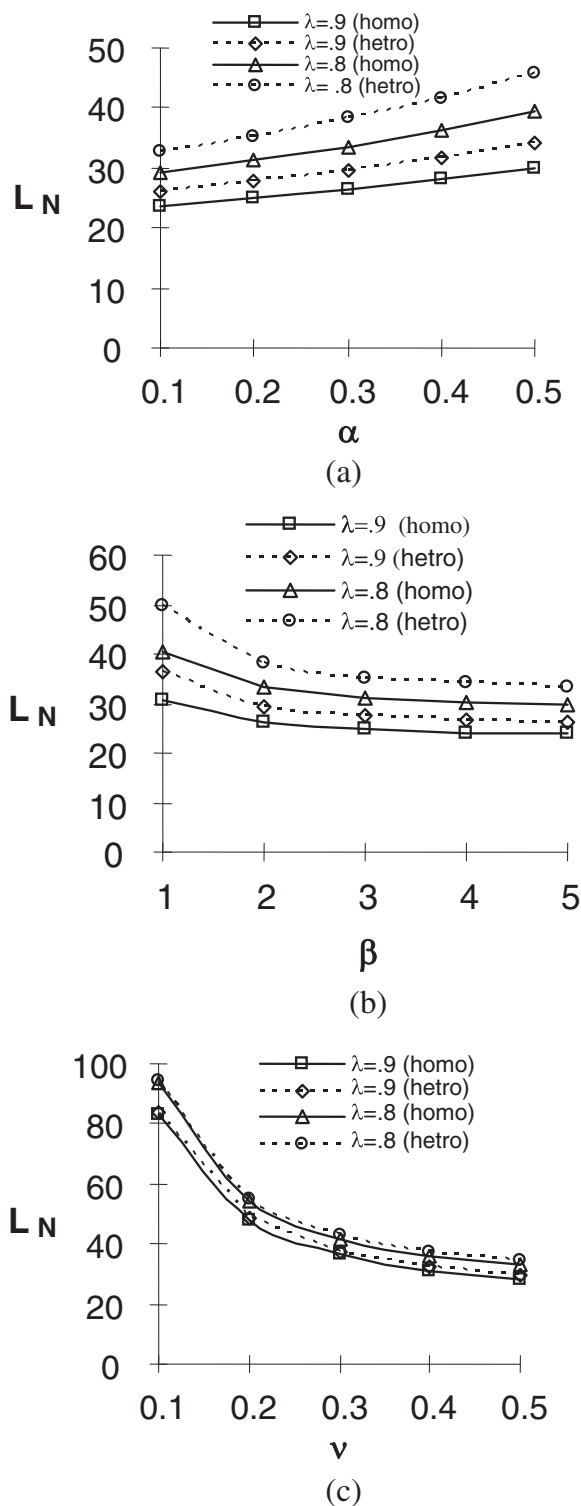
Figure 1 Average queue length vs. (a) \alpha , (b) \beta , and (c) v for homogeneous and heterogeneous arrival rates.
